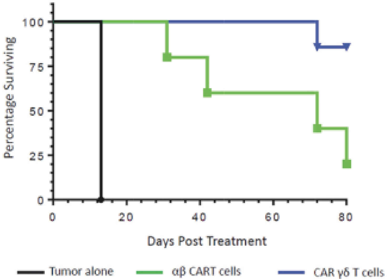
Figure 12. Anti-CD20 CAR gamma delta T cells do not induce GvHD, whereas treatment with anti-CD20 CAR alpha beta cells caused GvHD that led to increased mortality.
