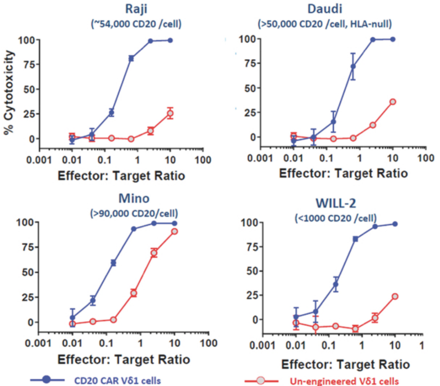
Figure 8. Anti-CD20 CAR gamma delta T cells demonstrated potent cell killing activity across multiple human tumor cell lines.
