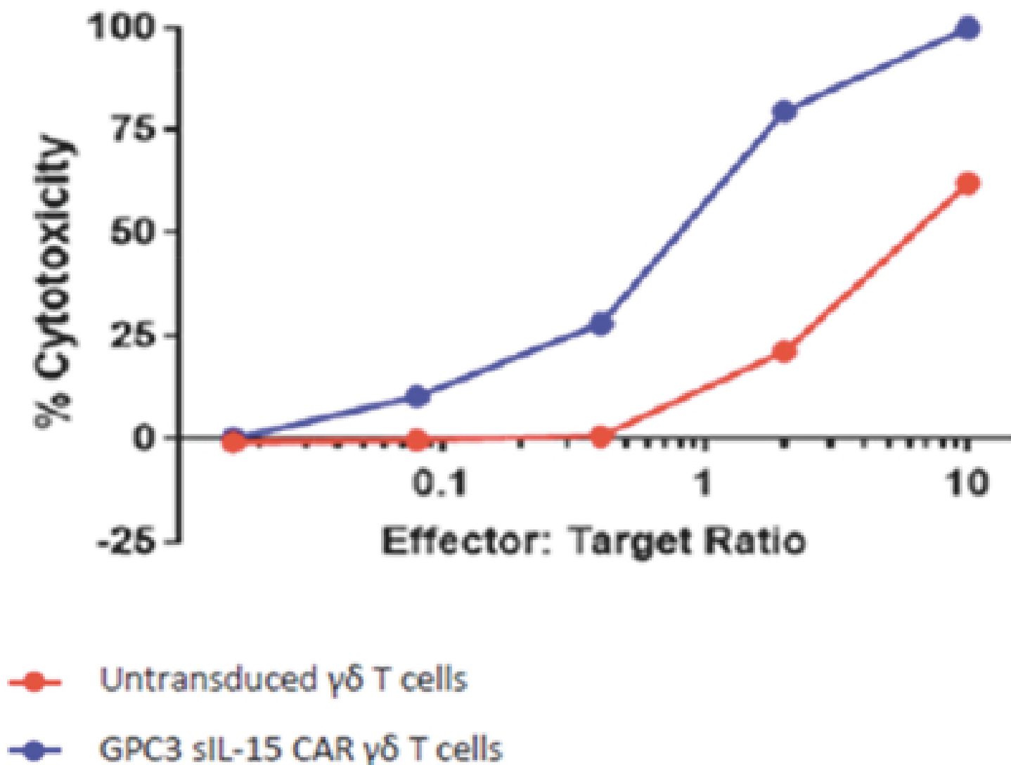
Figure 16. Expression of an anti-GPC3 CAR in gamma delta T cells led to potentiation of killing of HepG2 hepatocellular carcinoma cell line.
